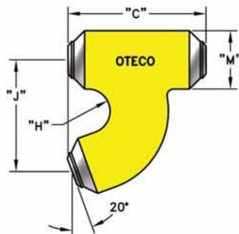
160° Standpipe Gooseneck with Top Outlet (GSNKTO)
