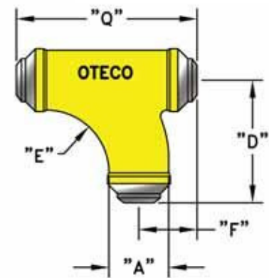
Long Sweep Tee (LST)
