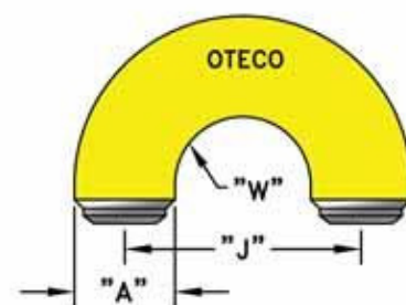
180° Standpipe Gooseneck (GSNK180)
