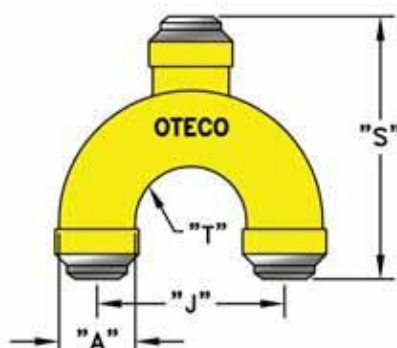
Long Sweep "Y" (LSY)
