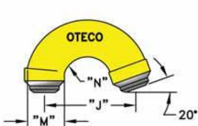
160° Standpipe Gooseneck (GSNK160)
