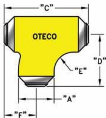
Long Sweep Tee (LST)
