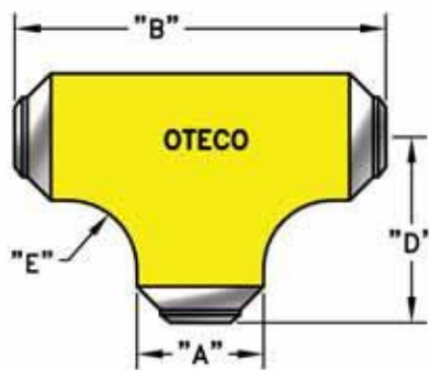
Long Sweep Full Flow Tee (LSFFT)
