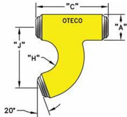
160° Standpipe Gooseneck with Top Outlet (GSNKTO)
