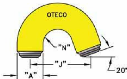
160° Standpipe Gooseneck (GSNK160)
