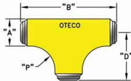
Long Sweep Full Flow Tee (LSFFT)
