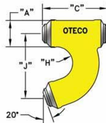
160° Standpipe Gooseneck with Top Outlet (GSNKTO)
