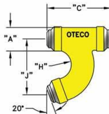
160° Standpipe Gooseneck with Top Outlet (GSNKTO)
