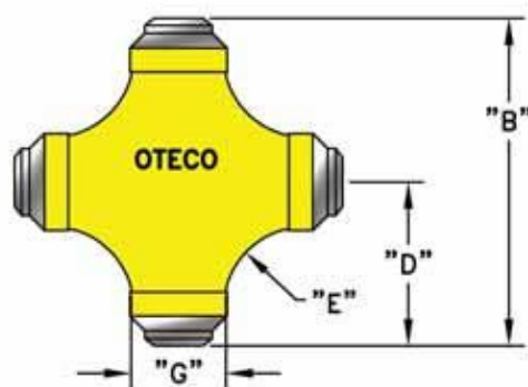
Full Flow Cross (FFC)
