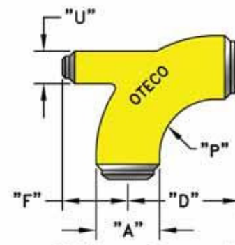
90° Long Sweep Ell with 2" Outlet (424LSE90)
