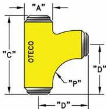
Long Sweep Tee (LST)
