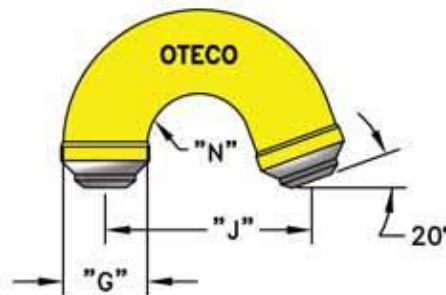
160° Standpipe Gooseneck (GSNK160)
