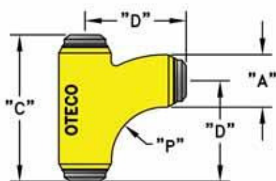
Long Sweep Tee (LST)
