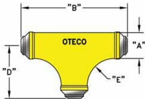
Long Sweep Full Flow Tee (LSFFT)
