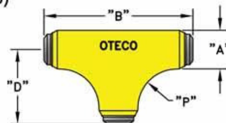
Long Sweep Full Flow Tee (LSFFT)
