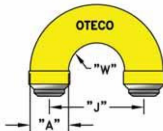
180° Standpipe Gooseneck (GSNK180)
